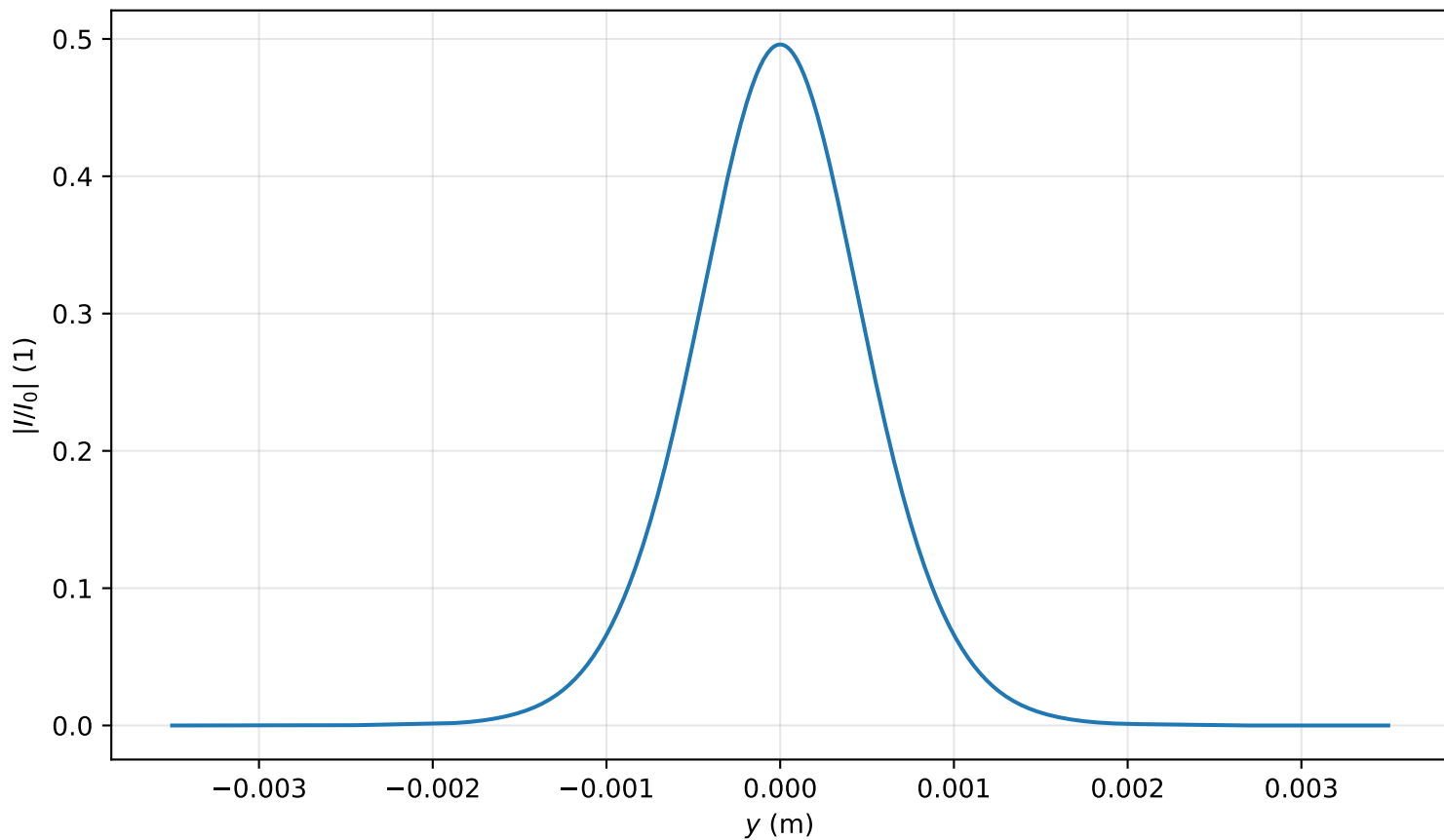
Intensity profile I(x=0, y, z=3.344)/I_0 , \text{Pin}=0.5\text{Pcr} , artificial time
